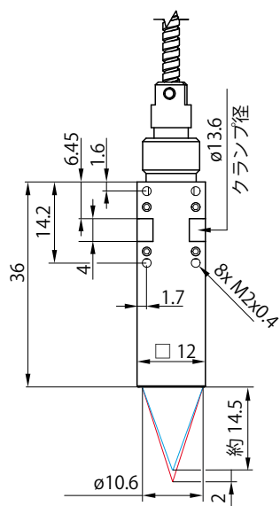
IFS2407-2HT/VAC
