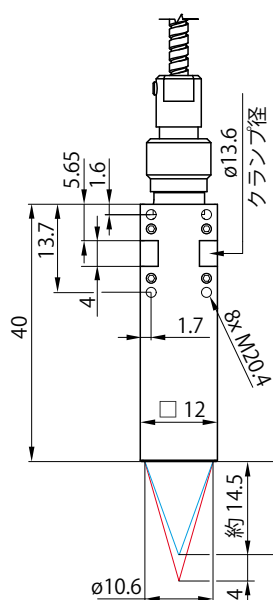
IFS2407-4HT/VAC
