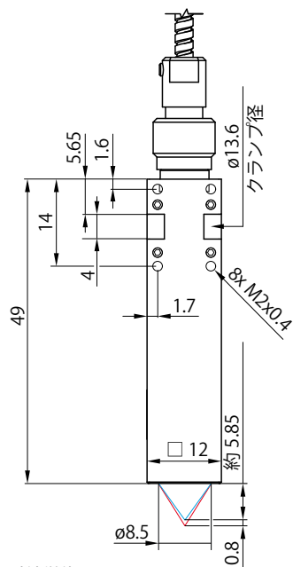
IFS2407-0.8HT/VAC
