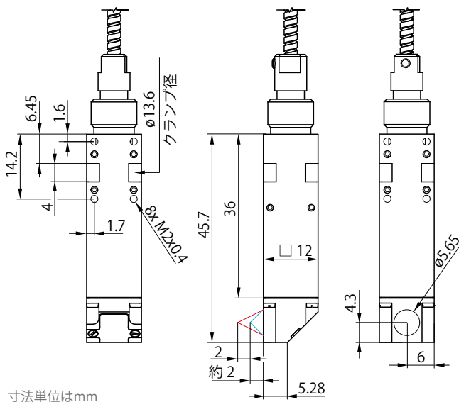
IFS2407/90-2HT/VAC
