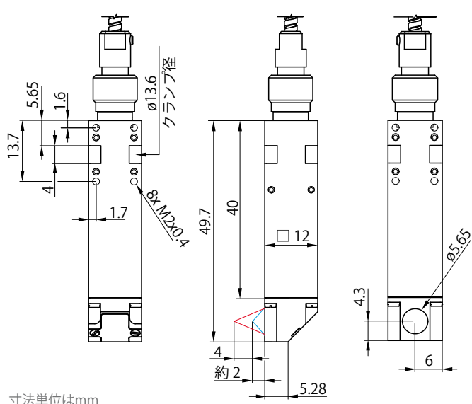
IFS2407/90-4HT/VAC
